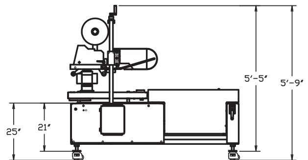
Dimensions shown of base machine only
